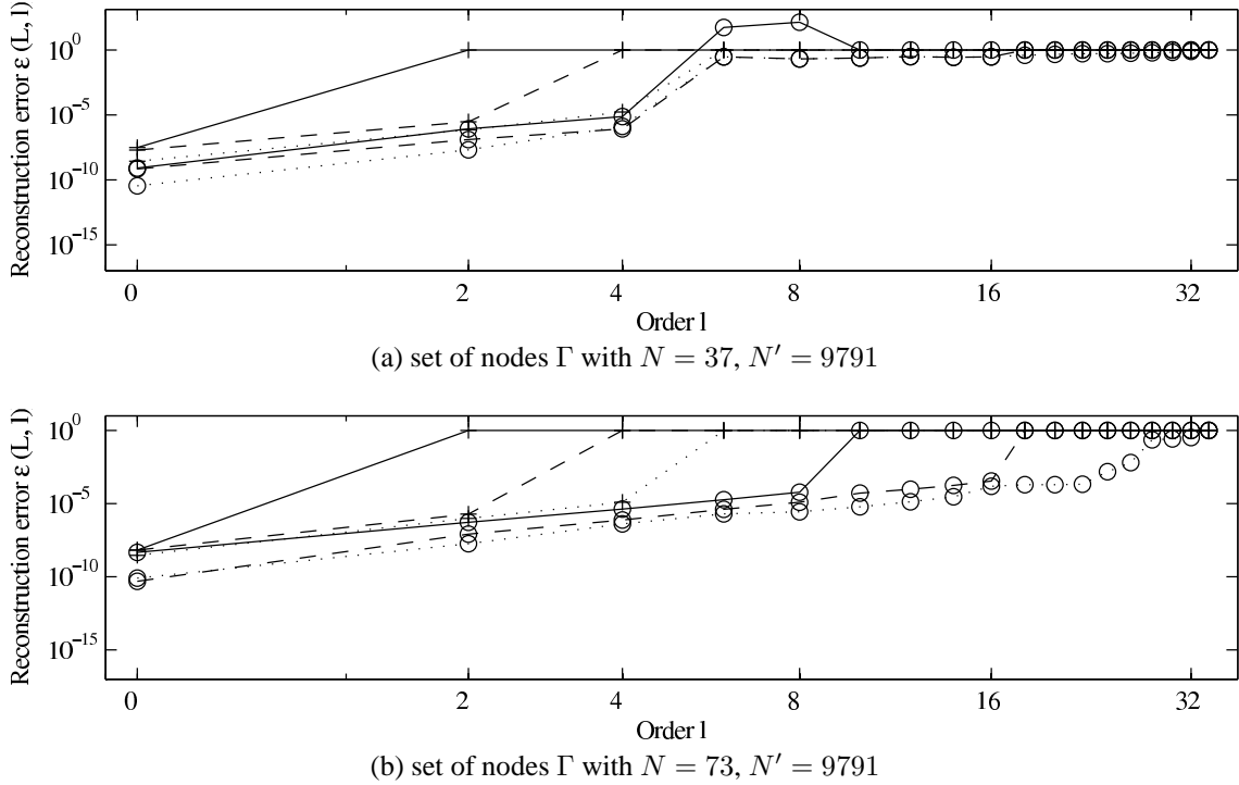
Figure 5.1: The approximation error \varepsilon(L, l) of the Fourier coefficients of a function with polynomial degree L_0 = 128 sampled at a set of nodes \Gamma in dependency of their order l and the total bandwidth used for approximation L = 0 (—+—), L = 2 (- - + -), L = 4 (· · · + · · ·), L = 8 (—○—), L = 16 (- - ○ -), L = 32 (· · · ○ · · ·).
